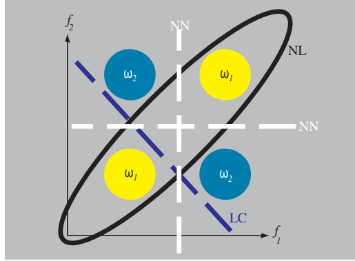
Figure 3. The yellow disks represent the locations of patterns in category \omega_1 in the two-dimensional feature space f_1 \times f_2 , and the dark-blue disks represent patterns in category \omega_2 . We assume these categories have equal prior probabilities, P(\omega_1) = P(\omega_2) = 0.5 . (This is an example of the exclusive-OR problem.) The projections of these probability densities onto the f_1 axis are the same for the two categories, and thus any classifier based solely on feature f_1 would have a 50% error rate, the worst possible for a dichotomizer where the categories have equal priors; that is, the Bayes error rate is 50%. Therefore, taken alone, measurements of f_1 of any test pattern are uninformative and useless for classification. The projection of the densities onto the other feature axis, f_2 , are similarly uninformative, and the classification rate based on feature f_2 alone is also 50%. Notice, though, that one particular classifier based on both features, shown by the (nonlinear) elliptical decision boundary marked NL, has 0% error rate—perfect classification. A nearest-neighbor classifier, marked NN, here would split the input space into quadrants, classifying all patterns in the upper-right and lower-left quadrants as \omega_1 and elsewhere \omega_2 , and thus also have a 0% error rate. Even a simple linear classifier, shown by the straight line marked LC, yields a 25% error rate. In short, even if f_1 represented some measure of the “fractal” properties of Pollock’s drip paintings, and even if taken alone provides no information for classification, this feature might be useful when used in a classifier based on multiple features.
